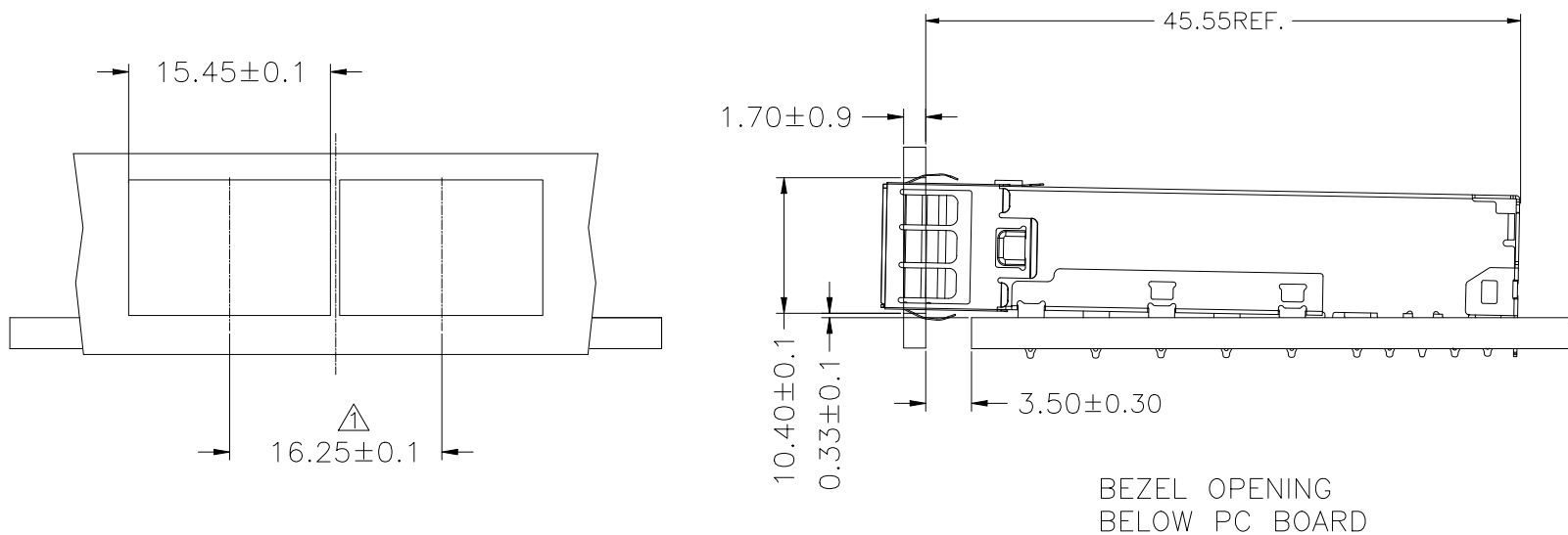
RECOMMENDED BEZEL DESIGN
