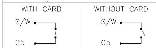
Circuit Diagram for Card Detect Switch
