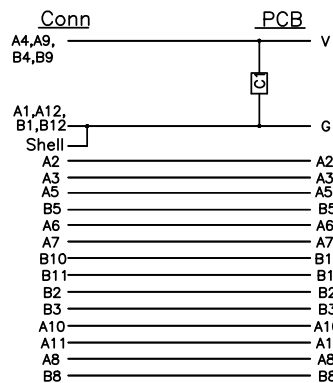
WIRE DIAGRAM
