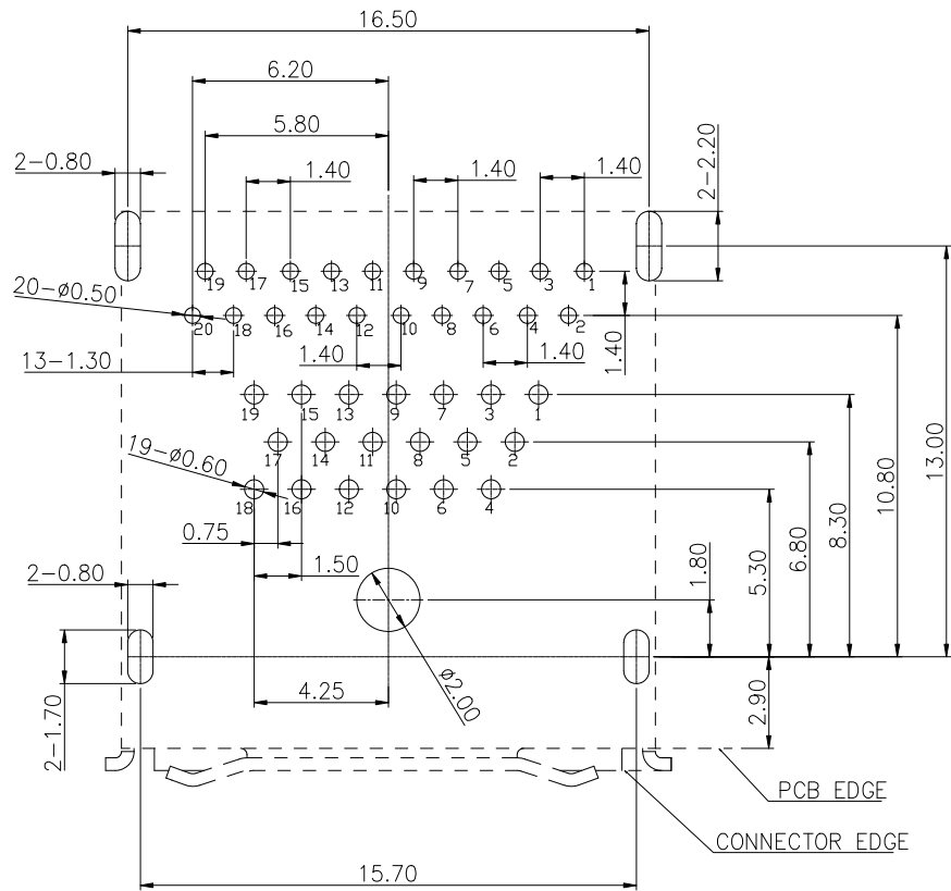
RECOMMENDED P.C.B LAYOUT(PCB THICKNESS: 1.6mm) COMPONENT SIDE VIEW(TOLERANCE: ±0.05)(SCALE: 2:1)
