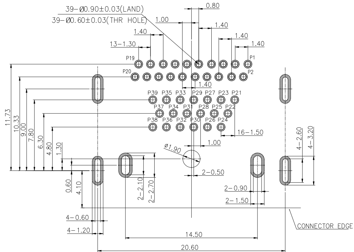
RECOMMENDED P.C.B LAYOUT(PCB THICKNESS: 1.6mm) COMPONENT SIDE VIEW(TOLERANCE: ±0.05)(SCALE: 2:1)
