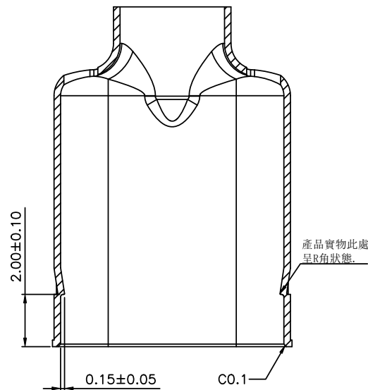
SECTION X-X
