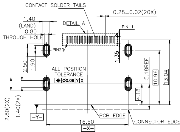
RECOMMENDED P.C.B LAYOUT (COMPONENT SIDE VIEW) PCB THICKNESS: 1.6mm TOLERANCE: ±0.05
