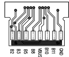
RECOMMENDED P.C.B LAYOUT TOP VIEW (TOLERANCE ±0.05mm)
