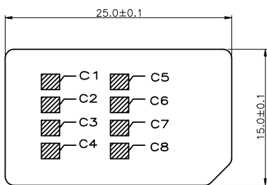
REFERENCE SIM CARD PLUG
