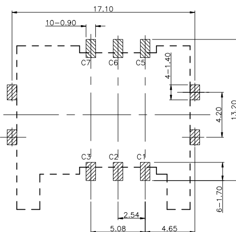
RECOMMENDED PCB MOUNTING PATTERN
