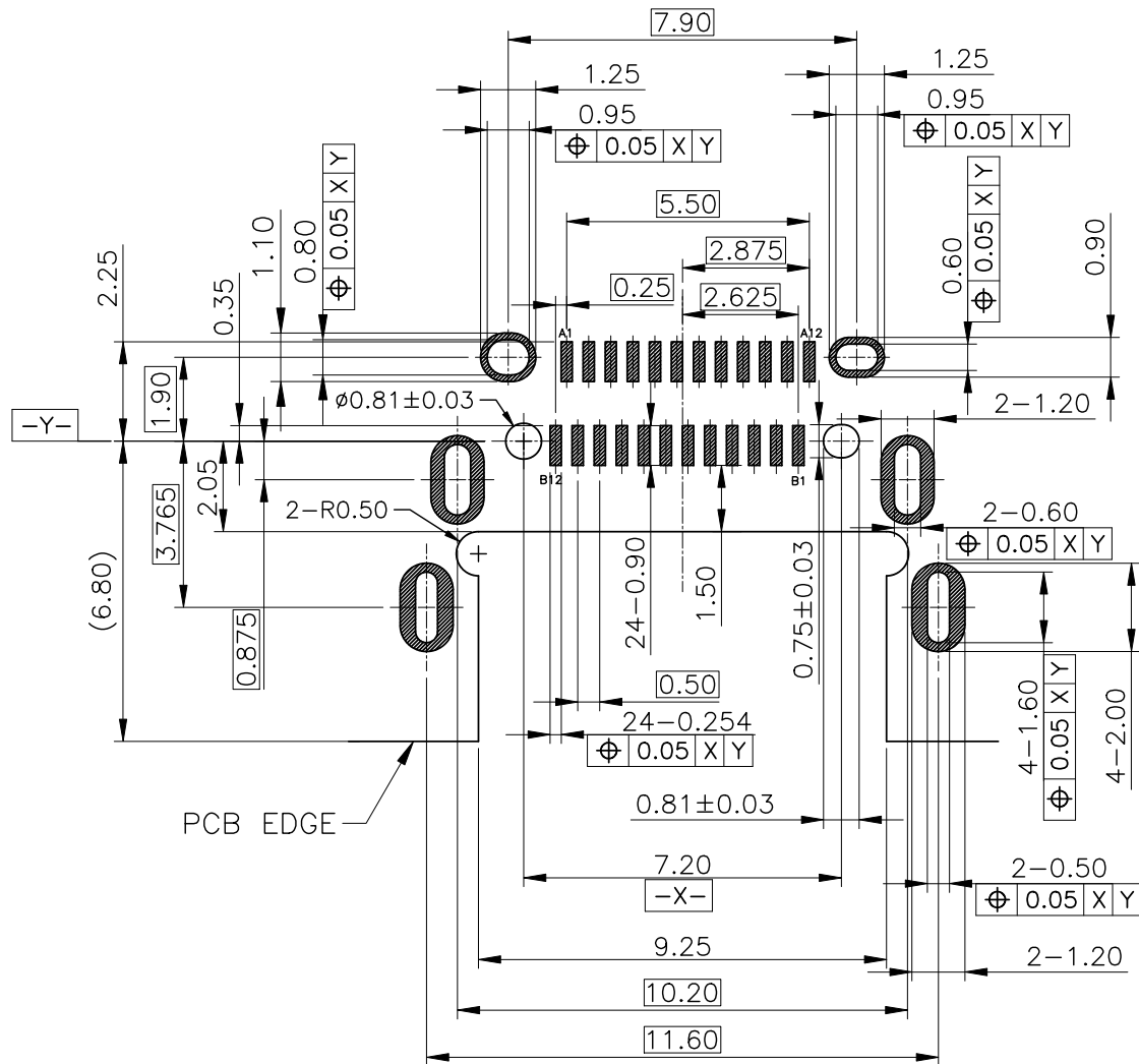
RECOMMENDED PCB LAYOUT(TOP VIEW) TOLERANCE:±0.05
