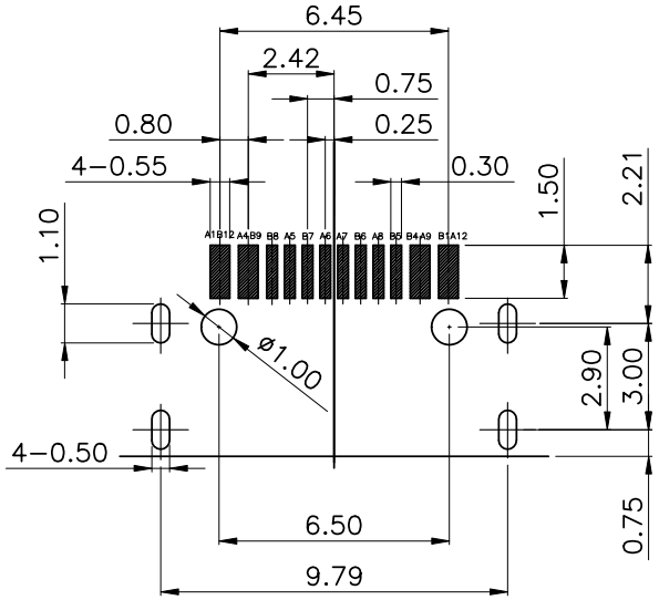
RECOMMENDED P.C.B. LAYOUT TOLERANCE UNSPECIFIED ±0.05mm
