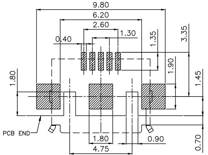
RECOMMENDED P.C. BOARD LAYOUT (TOLERANCE: ±0.05mm)
